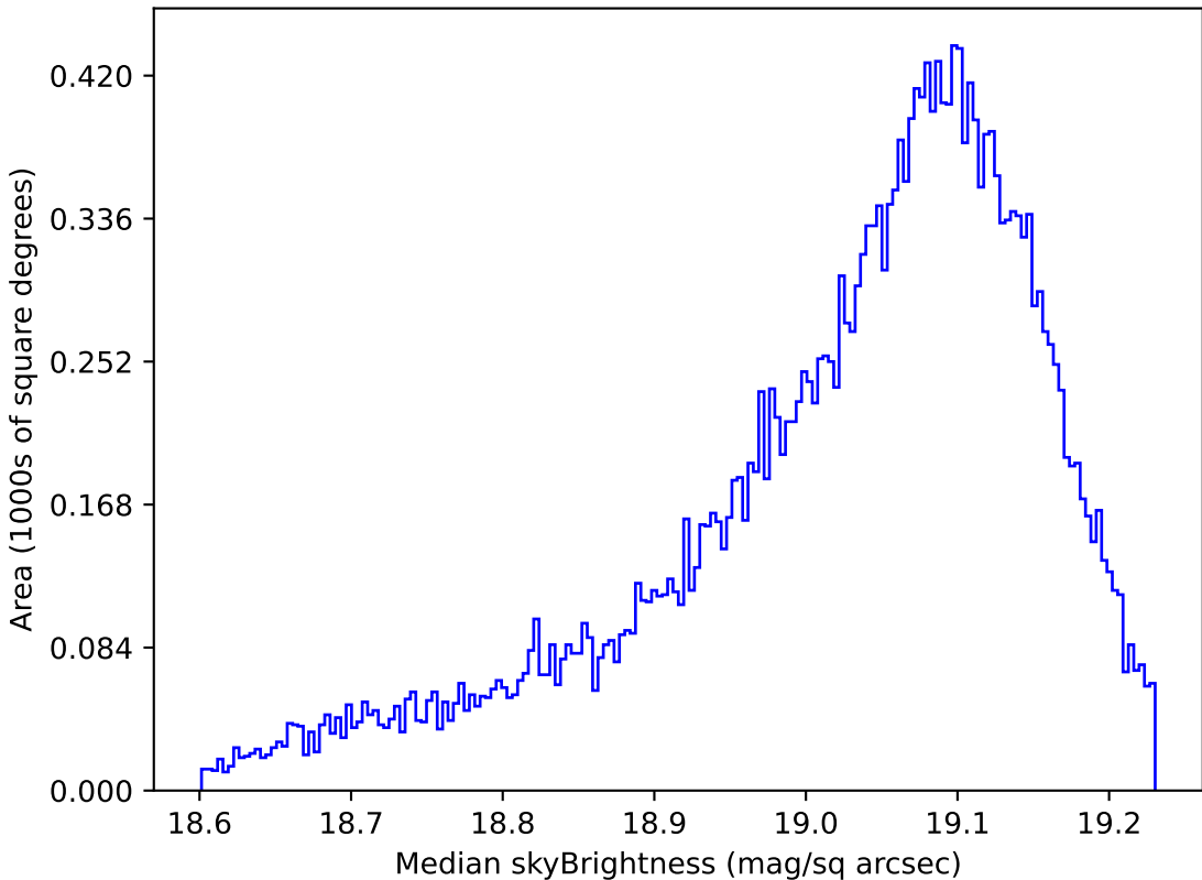
no_high_blob_v3.3_10yrs All sky z band: Median skyBrightness
