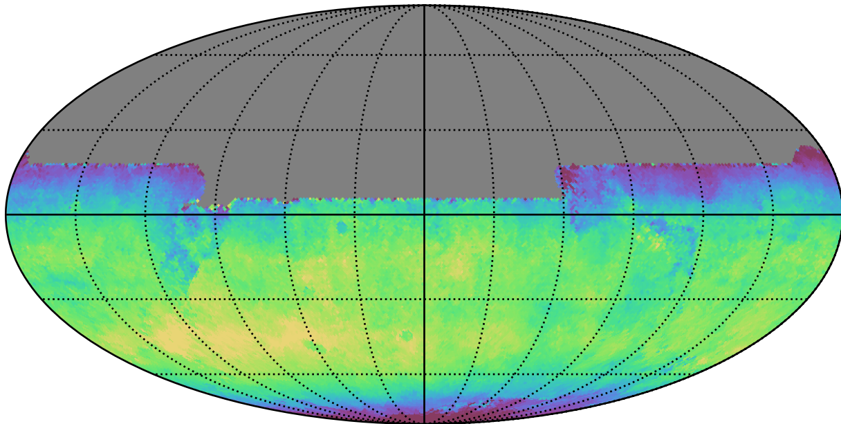
no_high_blob_v3.3_10yrs All sky y band: Median skyBrightness
