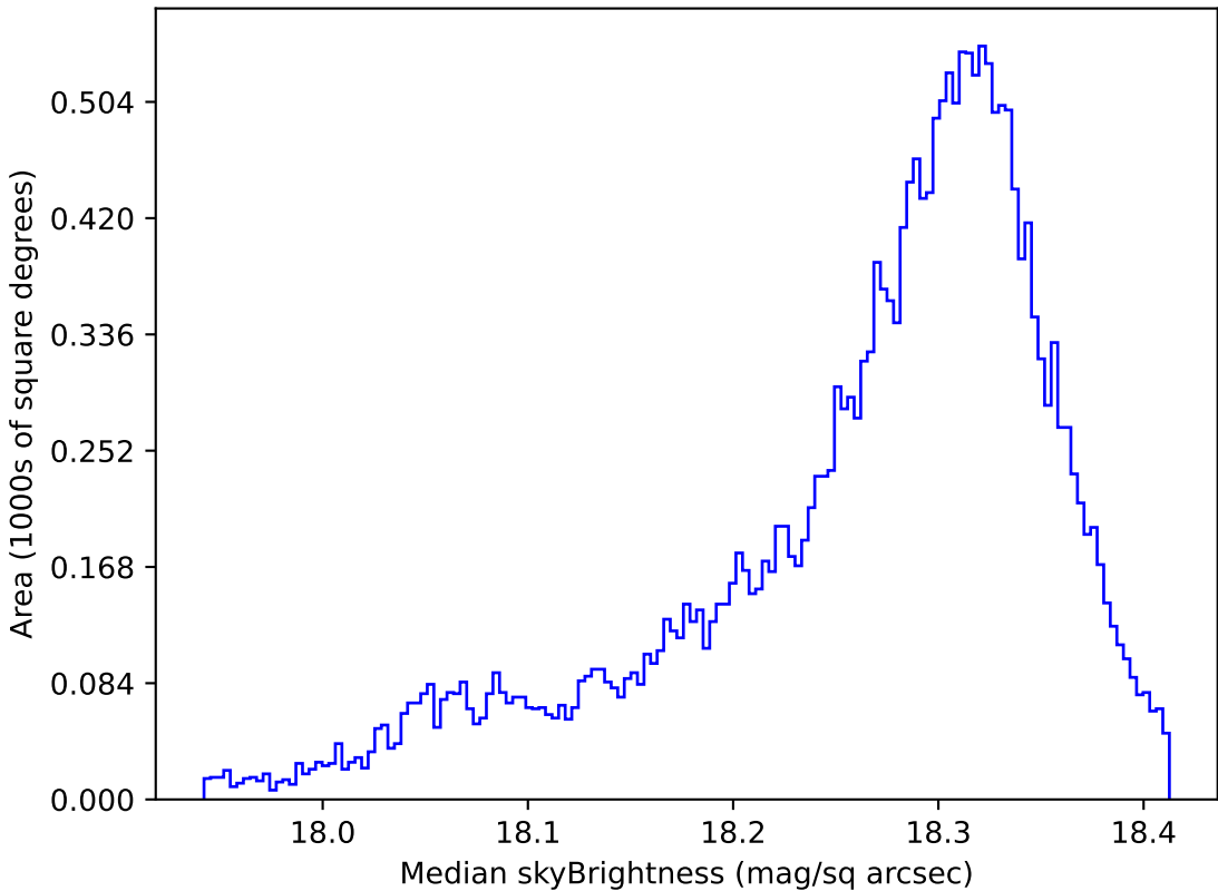
no_high_blob_v3.3_10yrs All sky y band: Median skyBrightness
