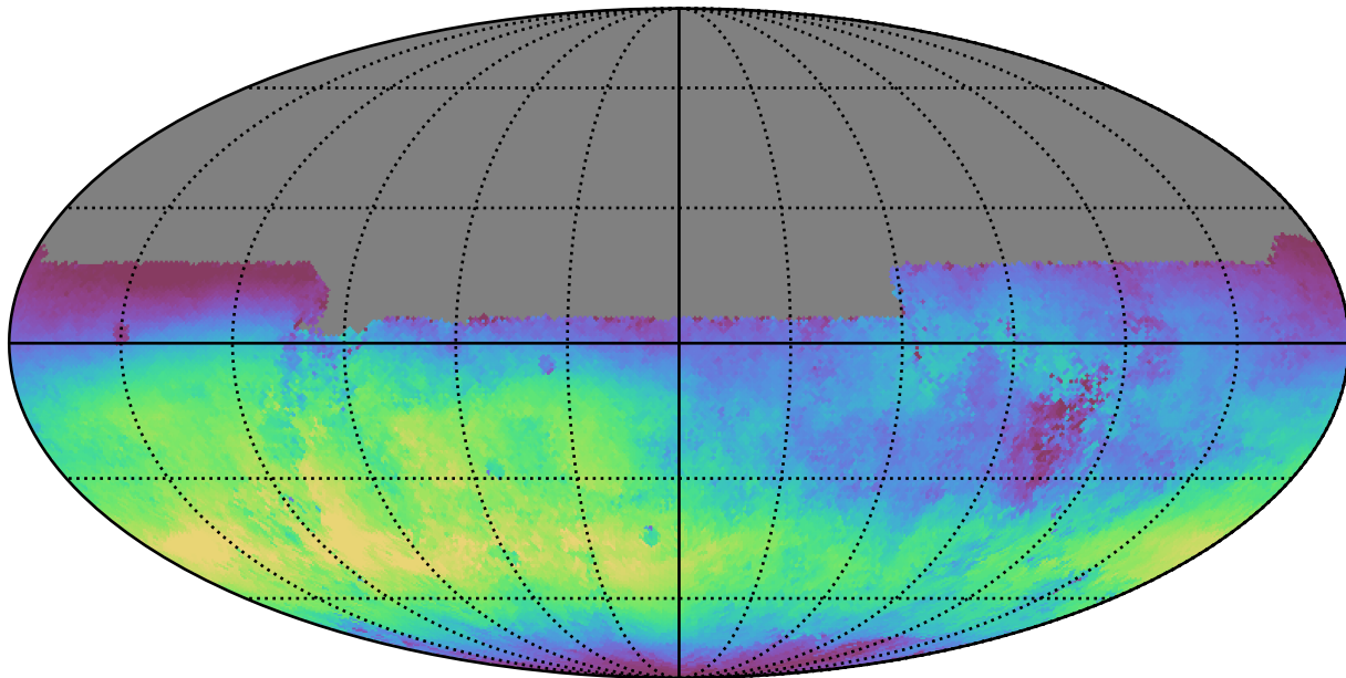
no_high_blob_v3.3_10yrs All sky u band: Median skyBrightness
