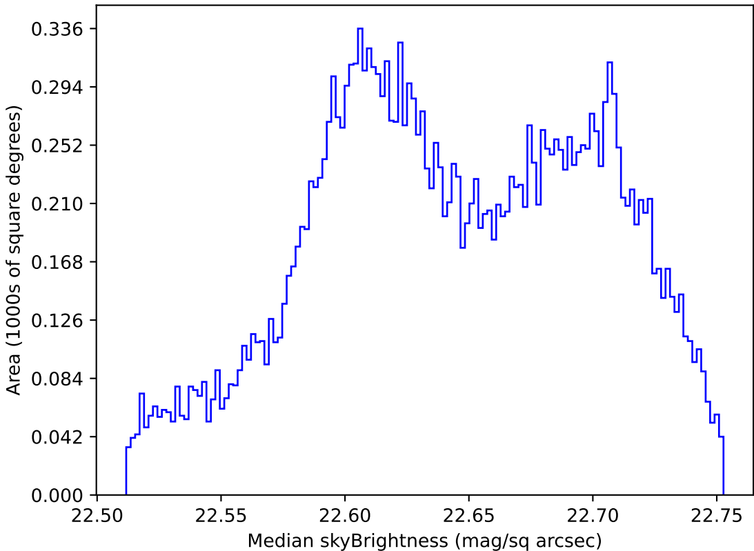
no_high_blob_v3.3_10yrs All sky u band: Median skyBrightness
