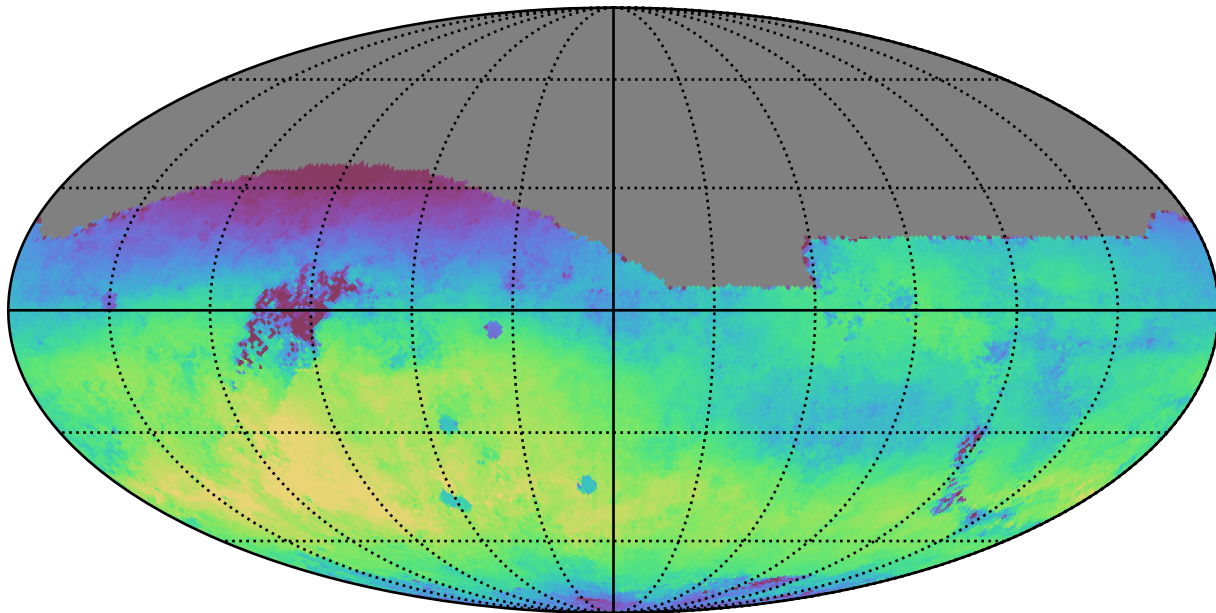
no_high_blob_v3.3_10yrs All sky r band: Median skyBrightness
