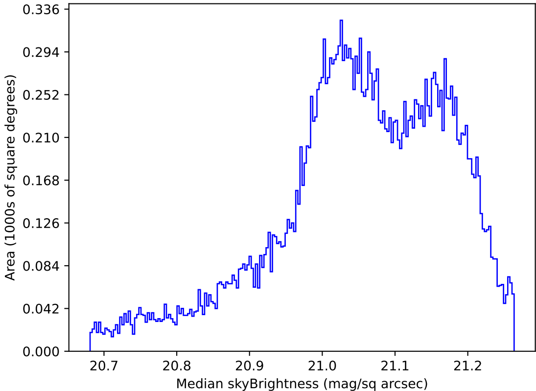
no_high_blob_v3.3_10yrs All sky r band: Median skyBrightness
