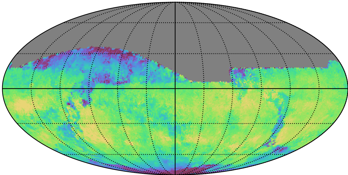
no_high_blob_v3.3_10yrs All sky i band: Median skyBrightness
