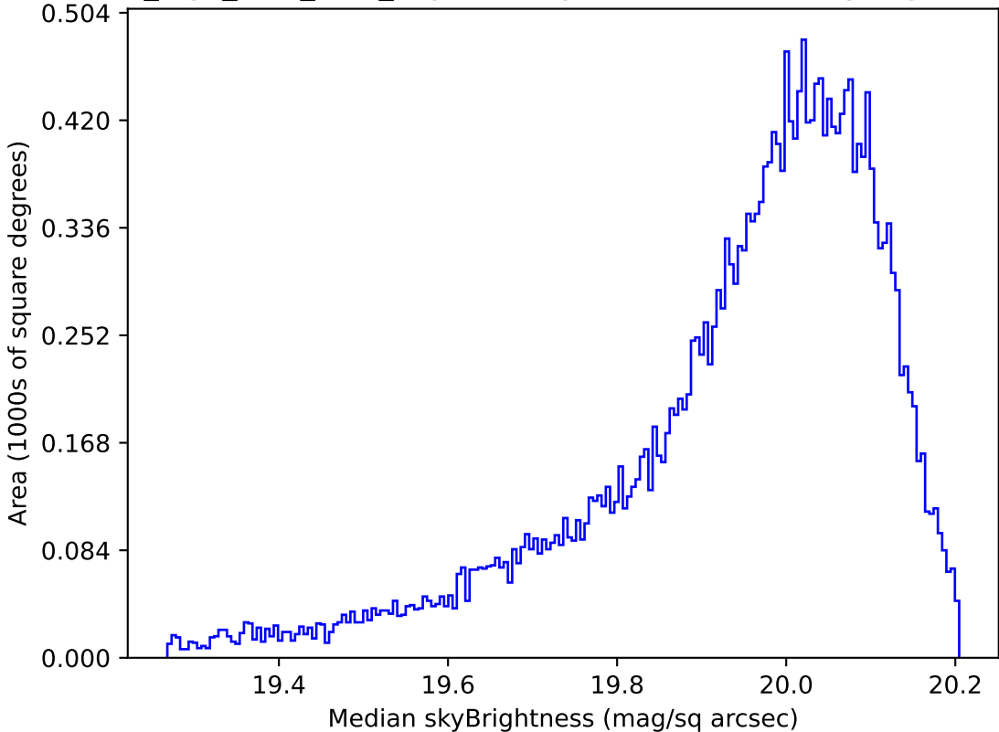
no_high_blob_v3.3_10yrs All sky i band: Median skyBrightness
