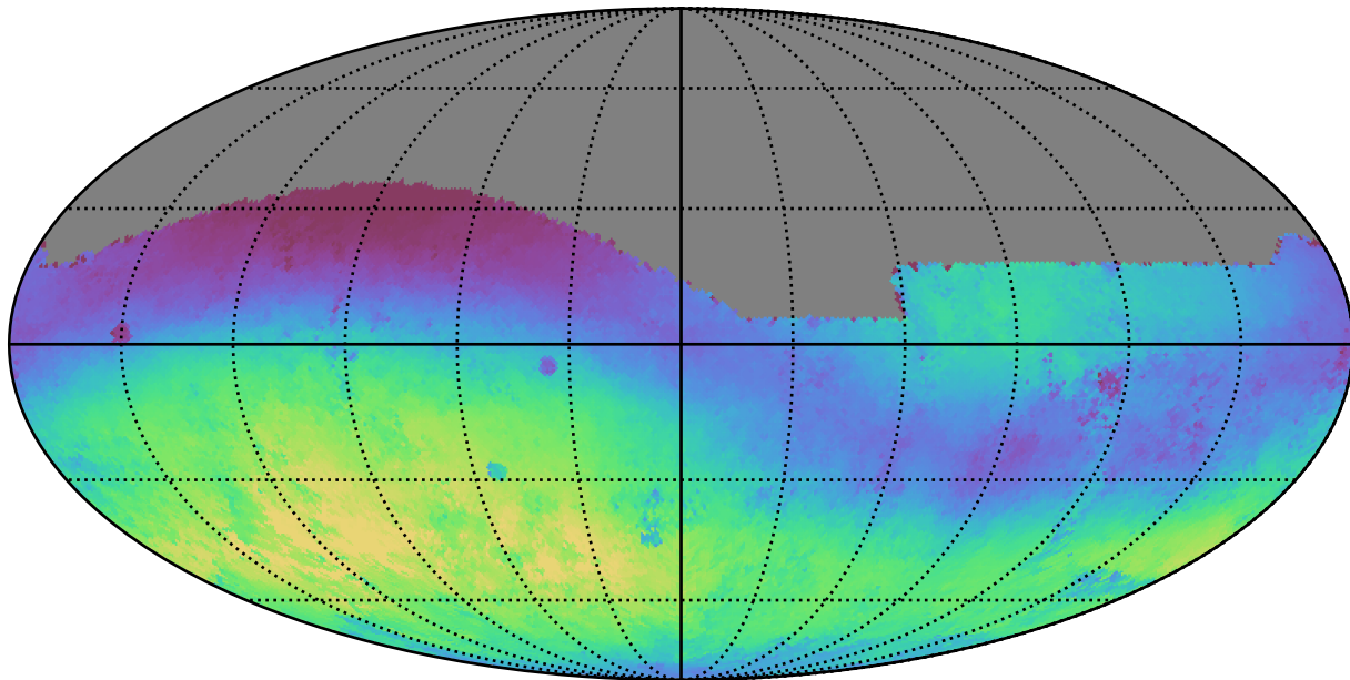
no_high_blob_v3.3_10yrs All sky g band: Median skyBrightness
