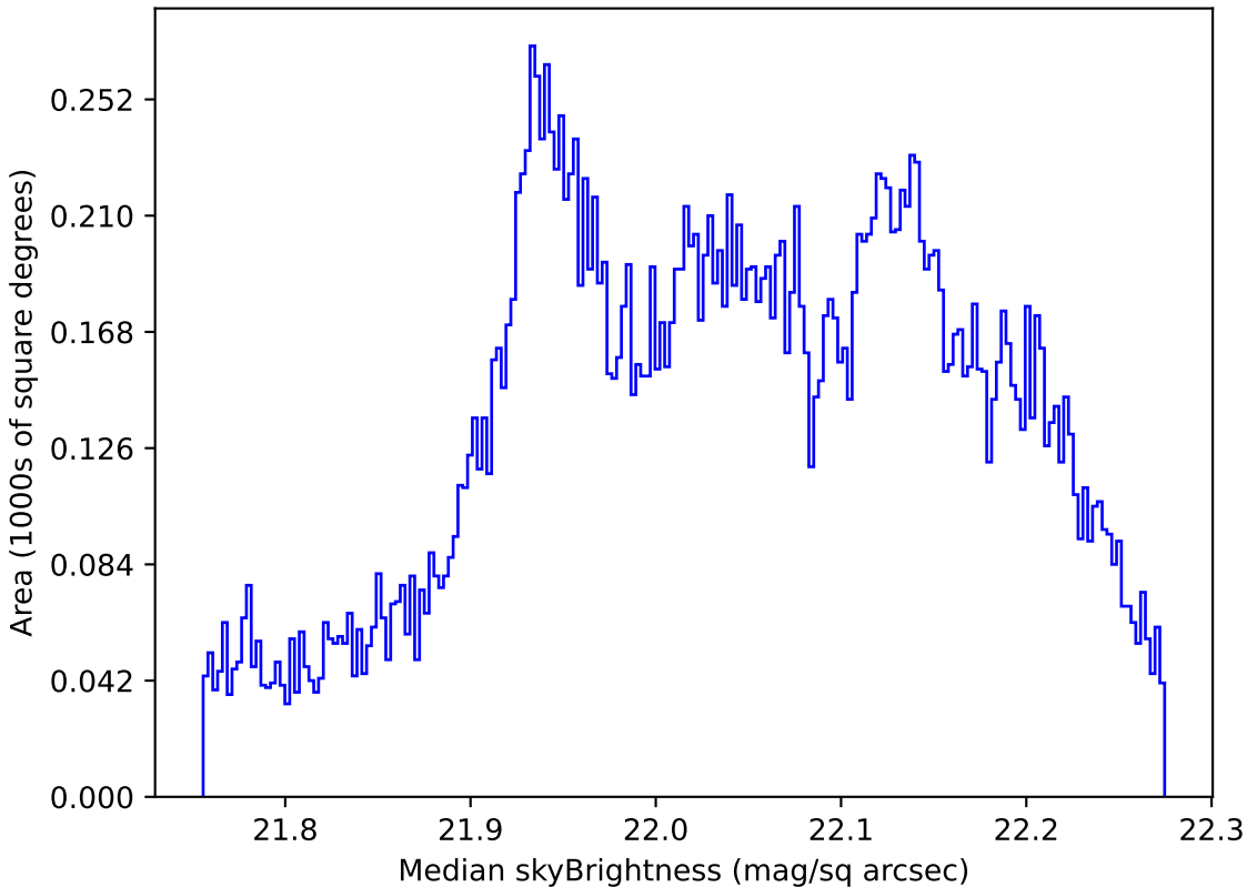
no_high_blob_v3.3_10yrs All sky g band: Median skyBrightness
