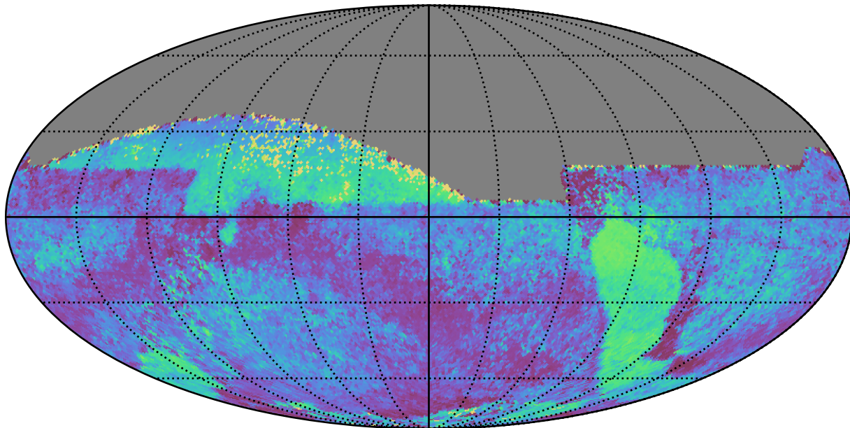
no_high_blob_v3.3_10yrs All sky all bands: Median skyBrightness
