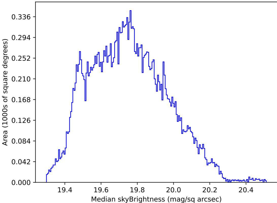
no_high_blob_v3.3_10yrs All sky all bands: Median skyBrightness
