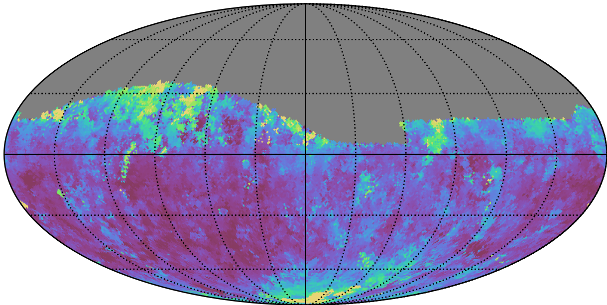
no_high_blob_v3.3_10yrs Yr 1 z band: Median seeingGeom
