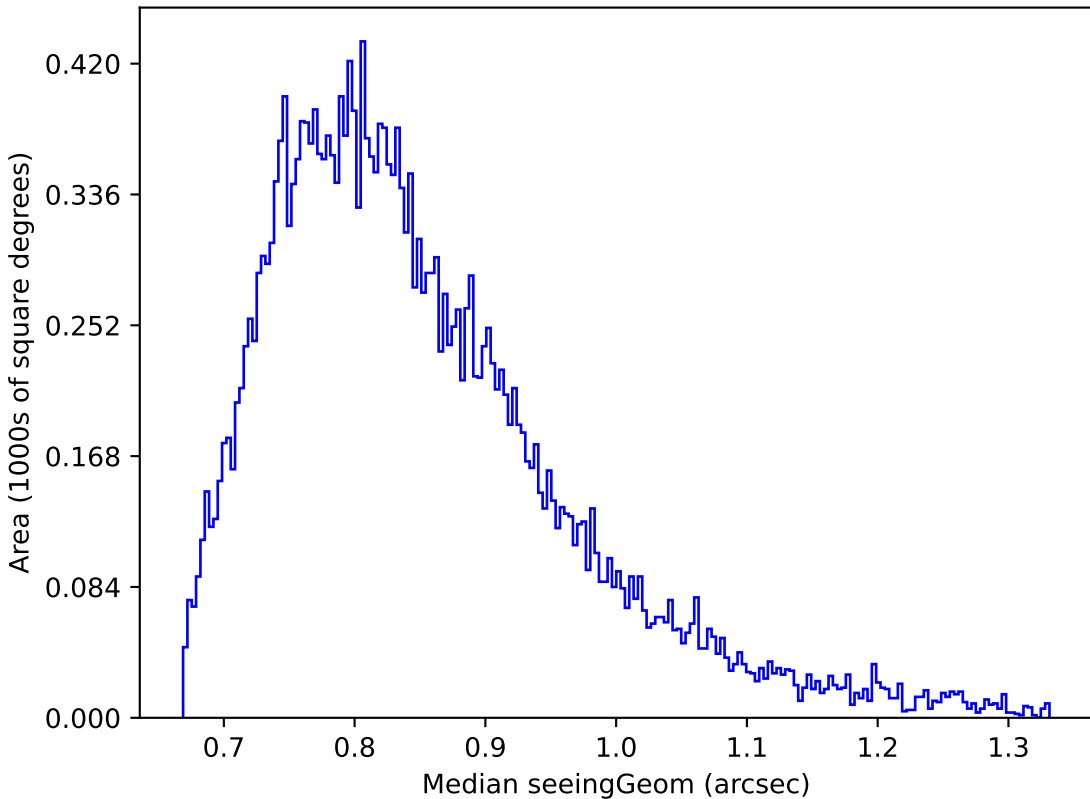
no_high_blob_v3.3_10yrs Yr 1 z band: Median seeingGeom
