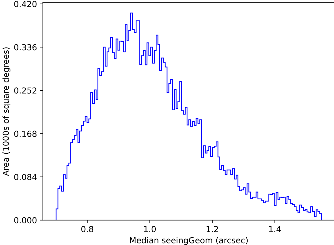
no_high_blob_v3.3_10yrs Yr 1 u band: Median seeingGeom
