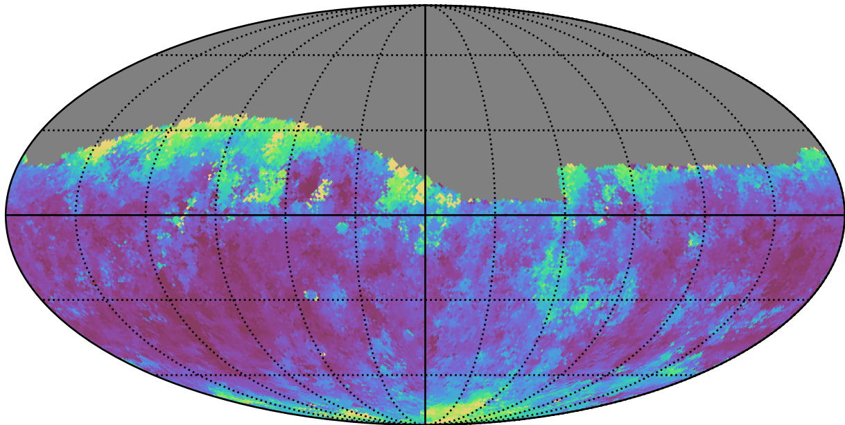
no_high_blob_v3.3_10yrs Yr 1 r band: Median seeingGeom
