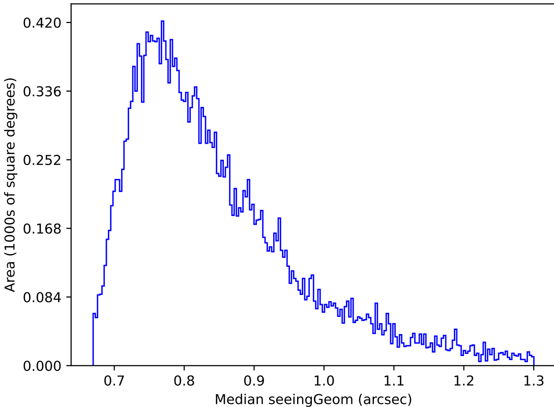
no_high_blob_v3.3_10yrs Yr 1 r band: Median seeingGeom
