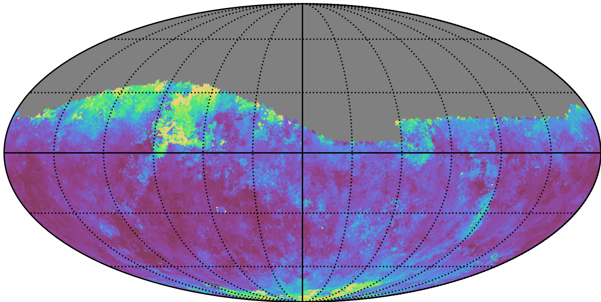
no_high_blob_v3.3_10yrs Yr 1 i band: Median seeingGeom
