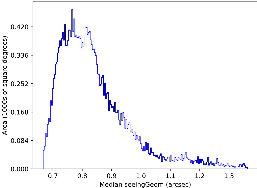
no_high_blob_v3.3_10yrs Yr 1 i band: Median seeingGeom
