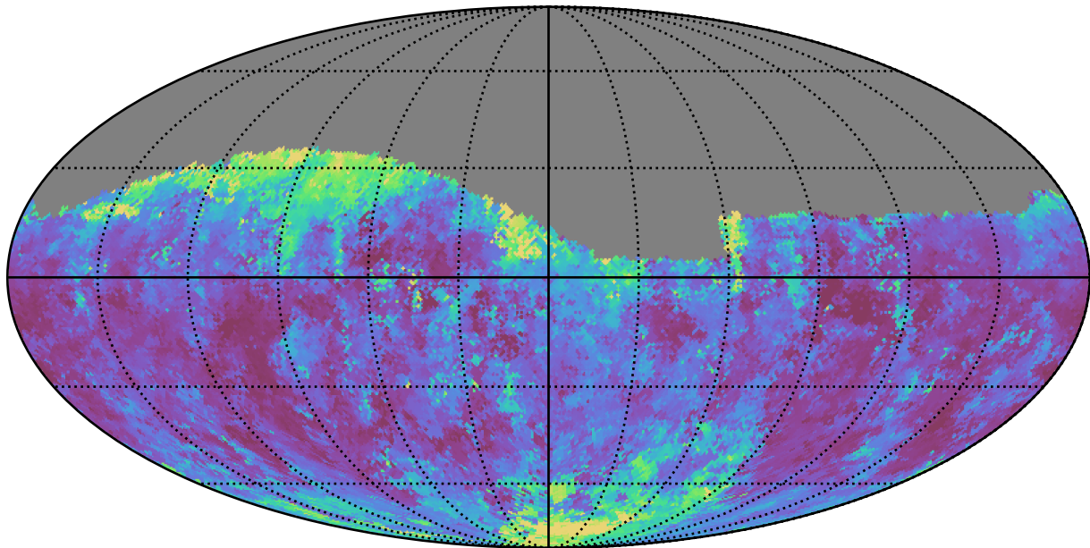
no_high_blob_v3.3_10yrs Yr 1 g band: Median seeingGeom
