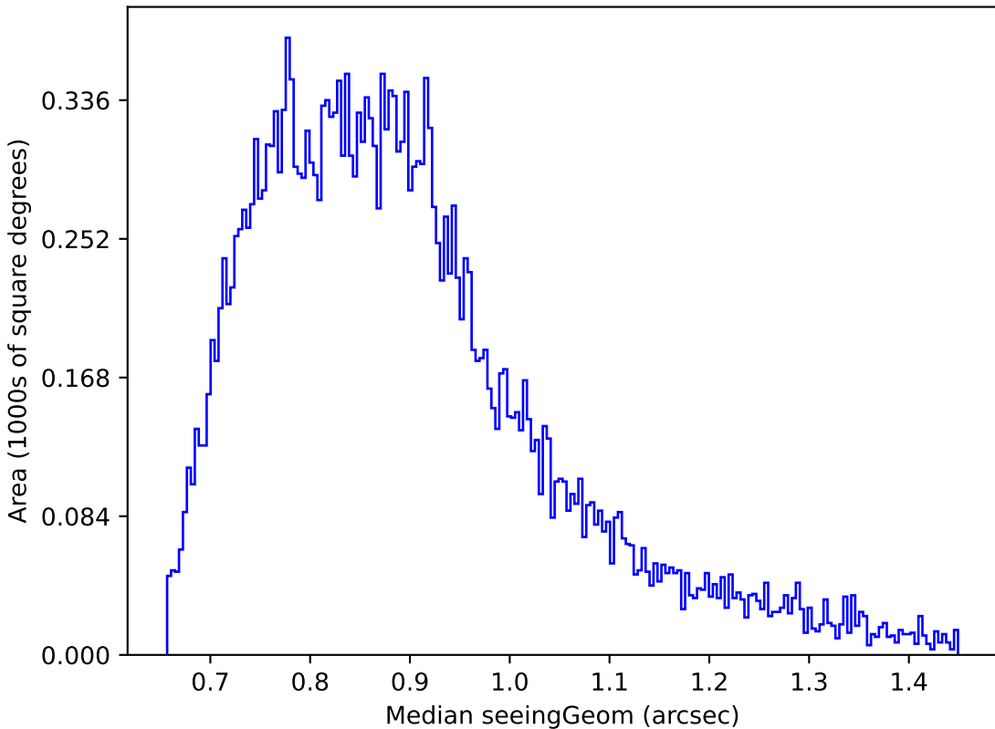
no_high_blob_v3.3_10yrs Yr 1 g band: Median seeingGeom
