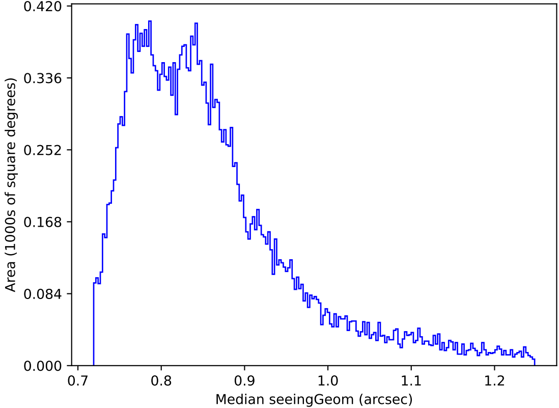
no_high_blob_v3.3_10yrs Yr 1 all bands: Median seeingGeom
