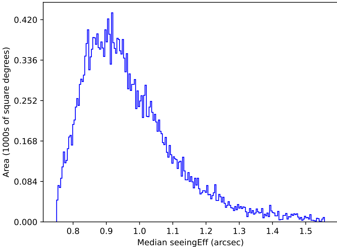
no_high_blob_v3.3_10yrs Yr 1 z band: Median seeingEff
