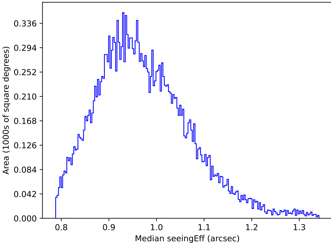
no_high_blob_v3.3_10yrs Yr 1 y band: Median seeingEff
