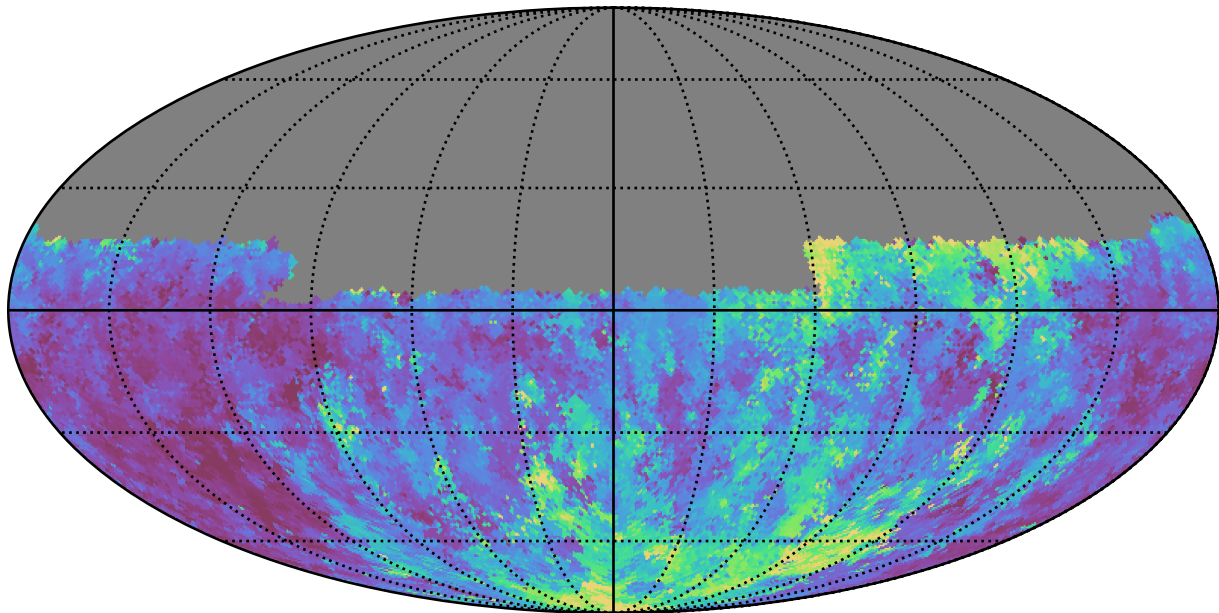
no_high_blob_v3.3_10yrs Yr 1 u band: Median seeingEff
