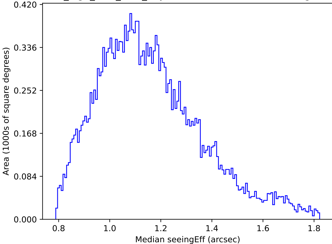
no_high_blob_v3.3_10yrs Yr 1 u band: Median seeingEff
