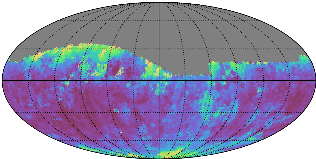
no_high_blob_v3.3_10yrs Yr 1 r band: Median seeingEff
