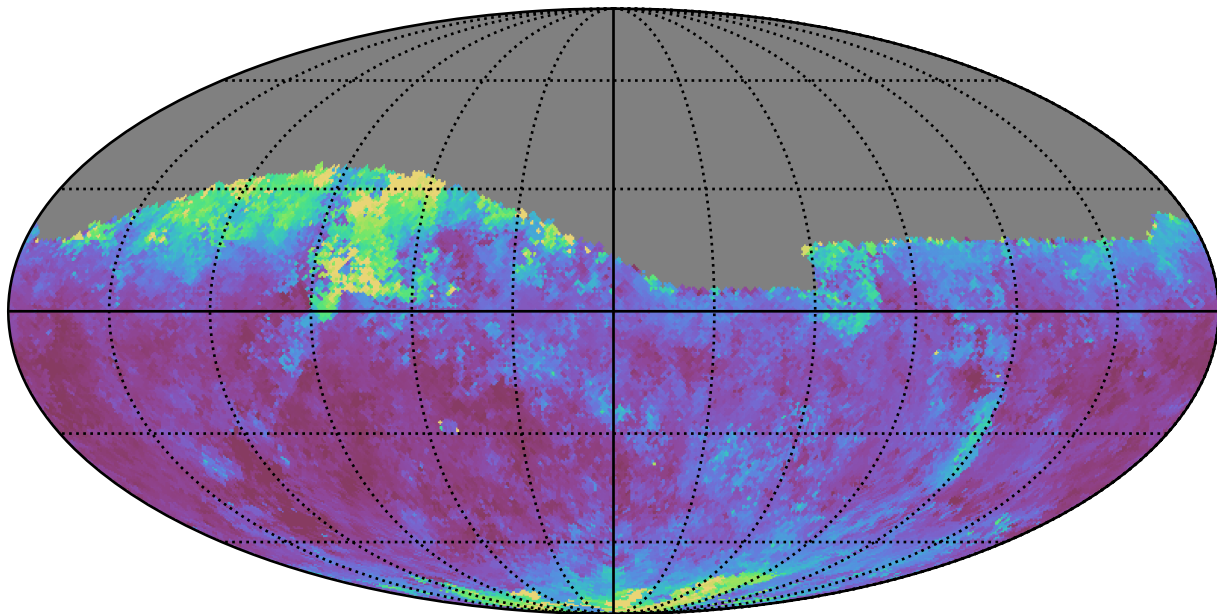
no_high_blob_v3.3_10yrs Yr 1 i band: Median seeingEff
