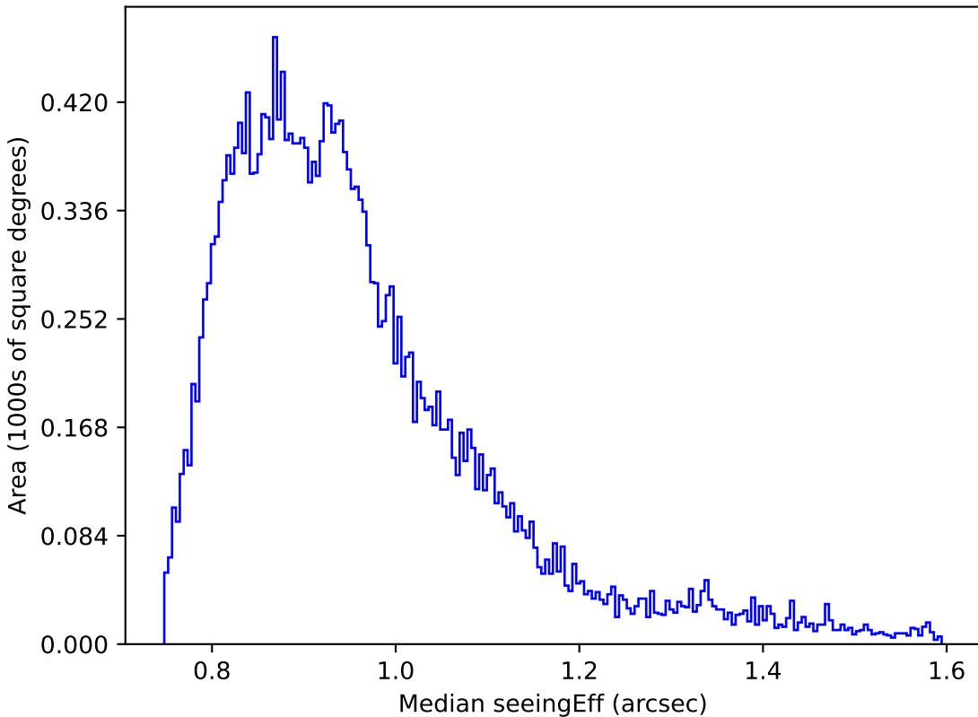
no_high_blob_v3.3_10yrs Yr 1 i band: Median seeingEff
