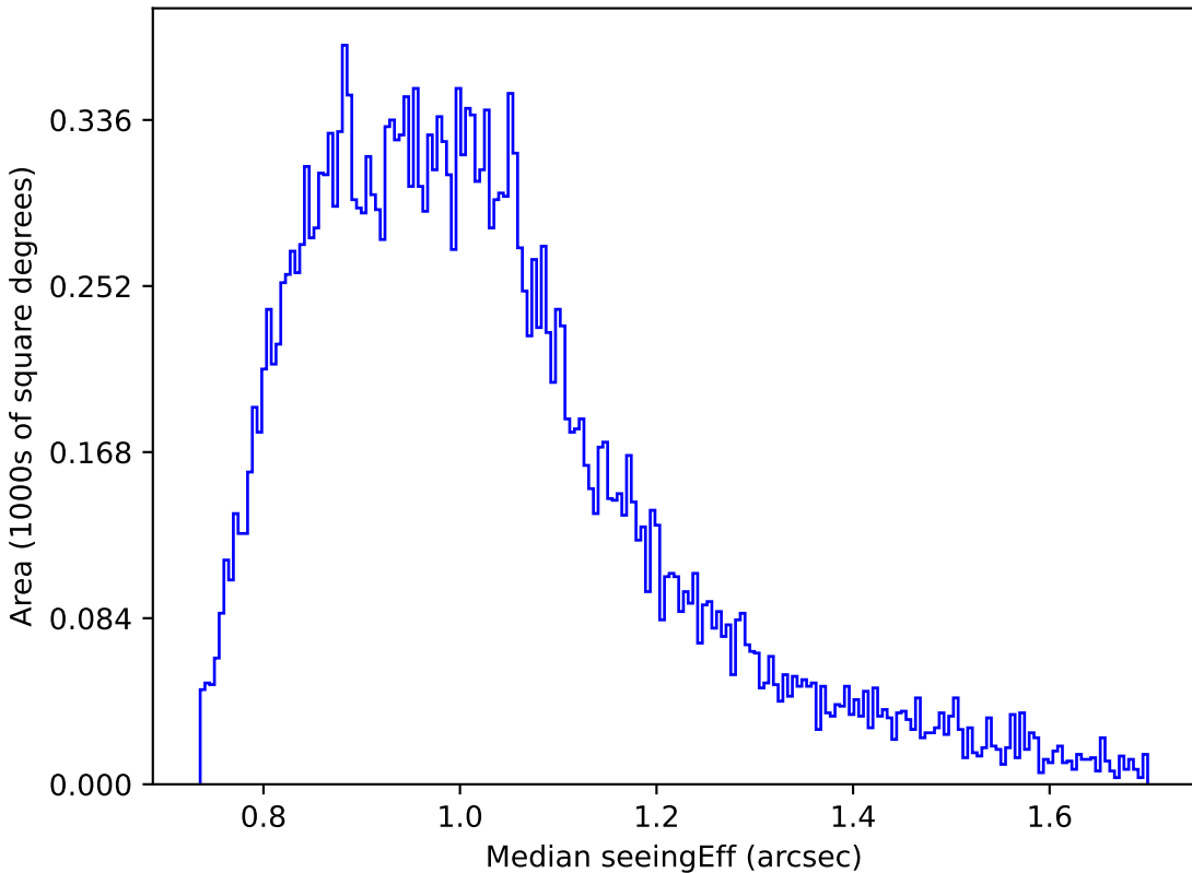
no_high_blob_v3.3_10yrs Yr 1 g band: Median seeingEff
