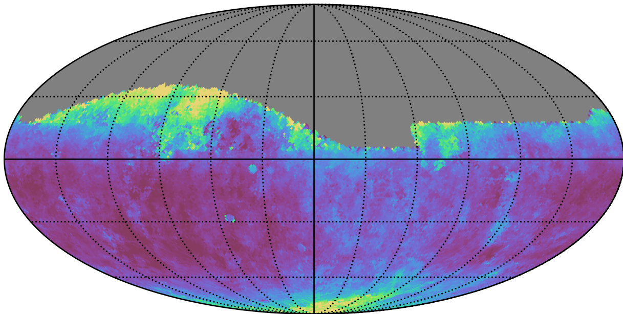
no_high_blob_v3.3_10yrs Yr 1 all bands: Median seeingEff
