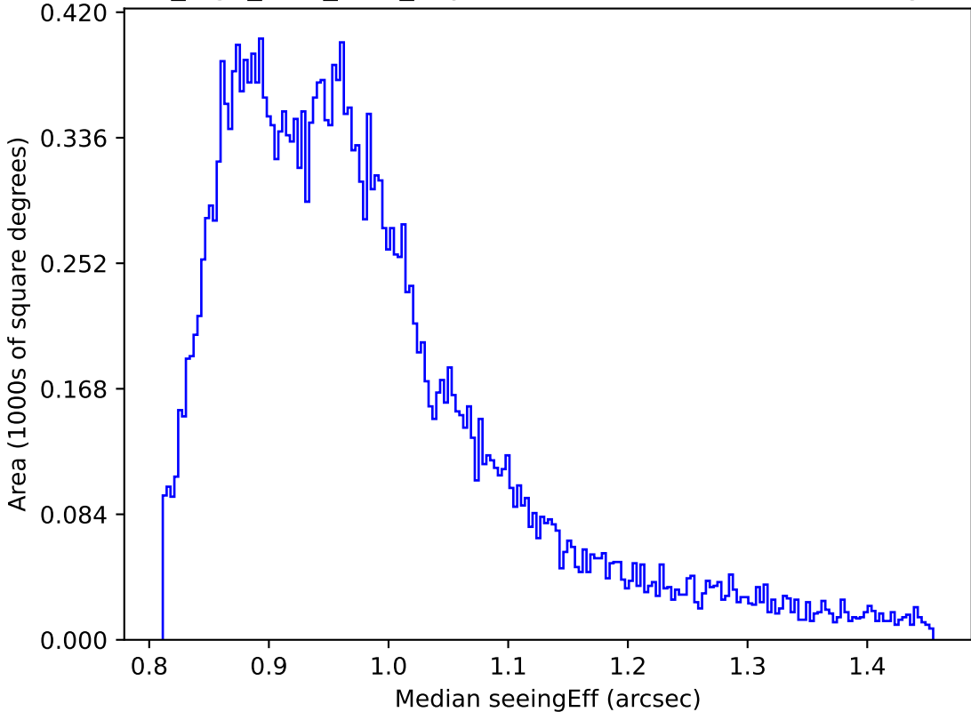
no_high_blob_v3.3_10yrs Yr 1 all bands: Median seeingEff
