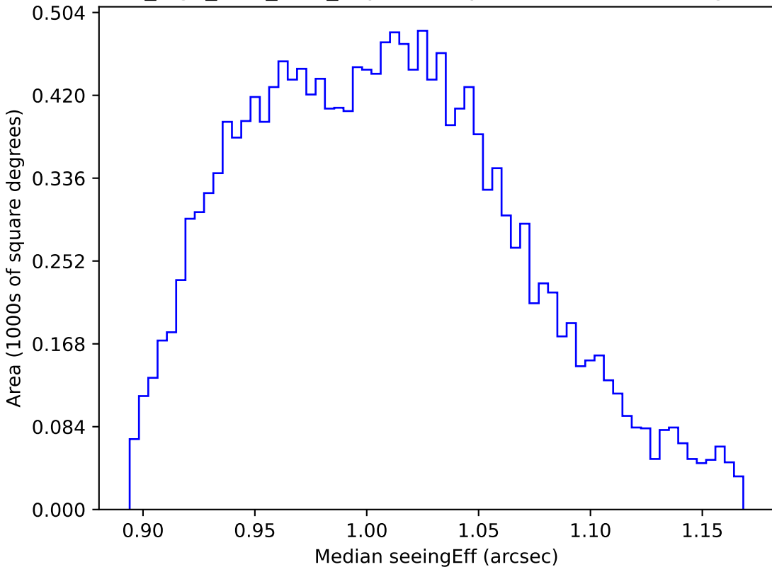
no_high_blob_v3.3_10yrs WFD y band: Median seeingEff
