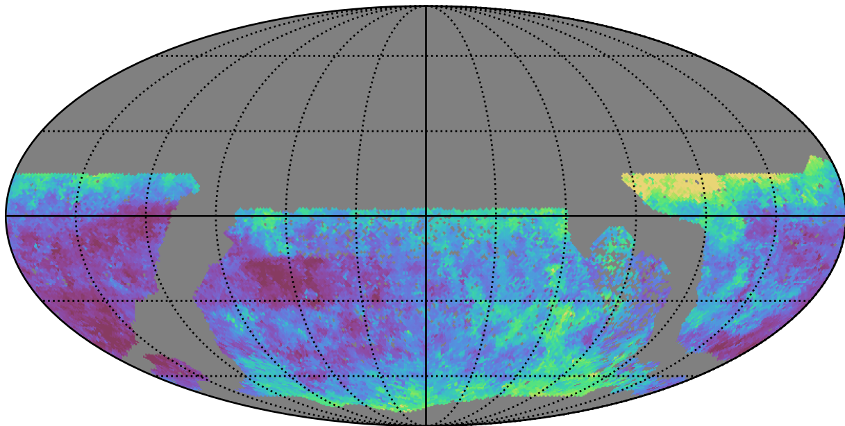
no_high_blob_v3.3_10yrs WFD u band: Median seeingEff
