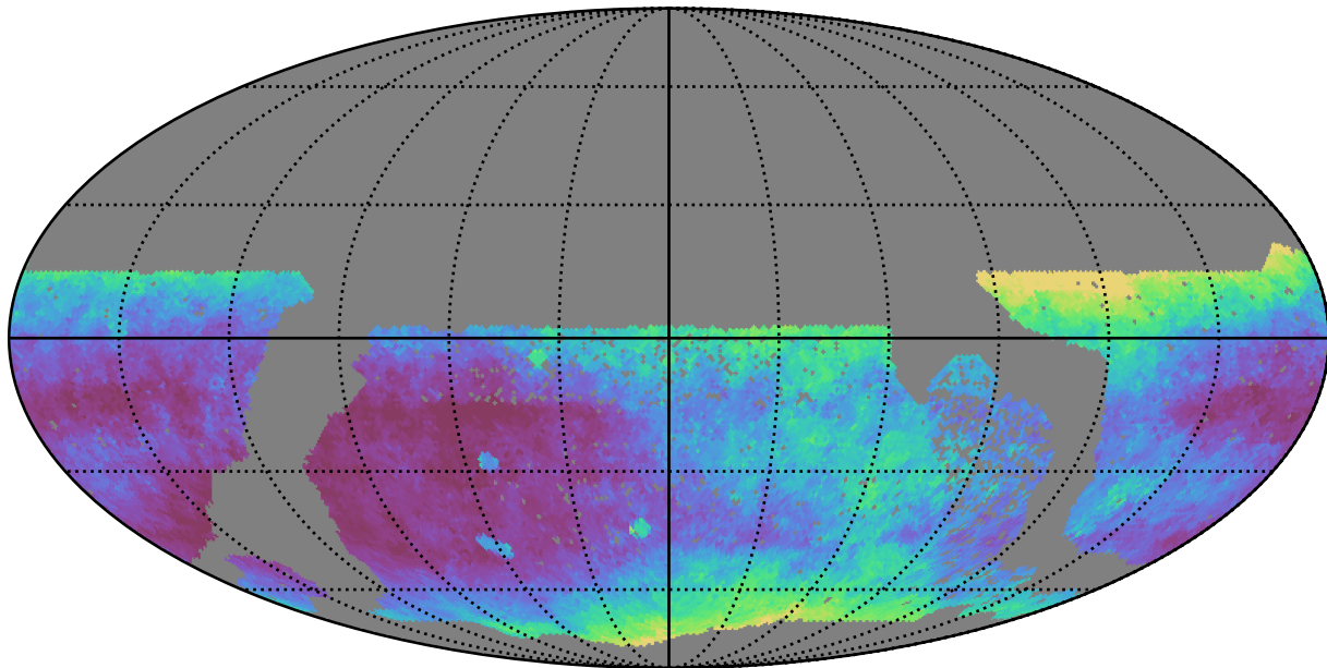
no_high_blob_v3.3_10yrs WFD r band: Median seeingEff
