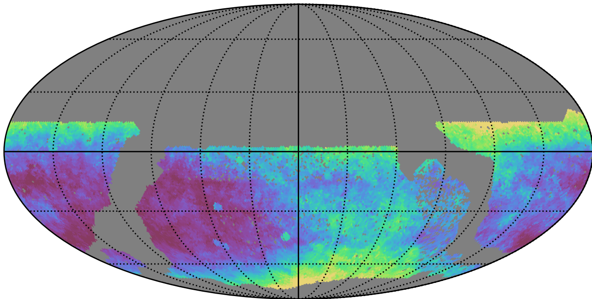
no_high_blob_v3.3_10yrs WFD i band: Median seeingEff
