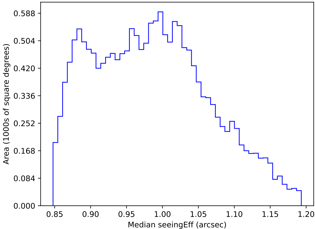
no_high_blob_v3.3_10yrs WFD i band: Median seeingEff
