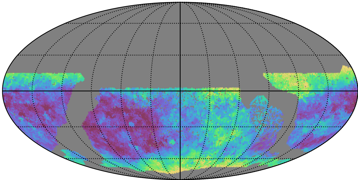
no_high_blob_v3.3_10yrs WFD g band: Median seeingEff
