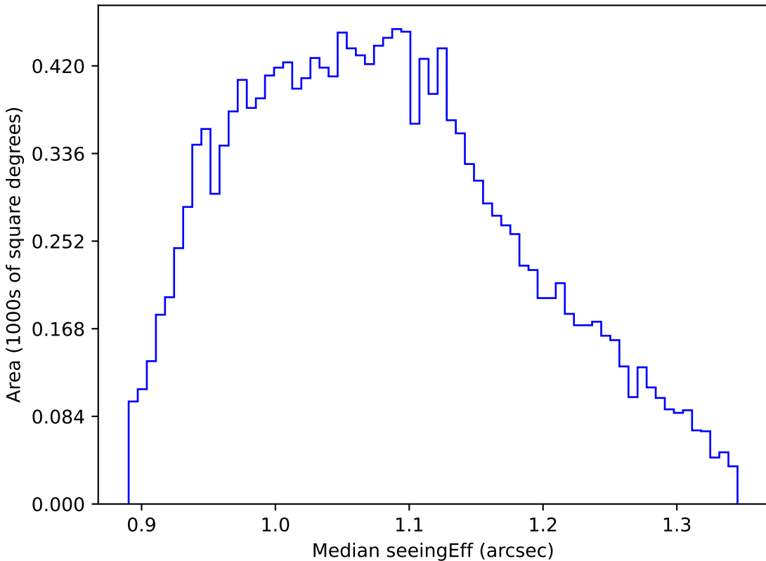
no_high_blob_v3.3_10yrs WFD g band: Median seeingEff
