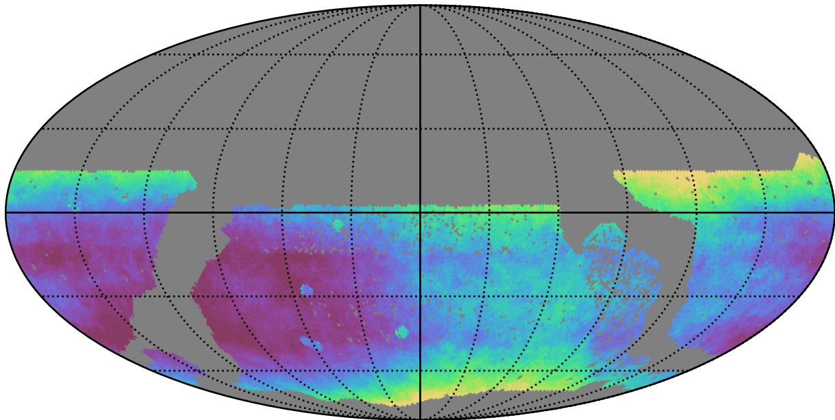
no_high_blob_v3.3_10yrs WFD all bands: Median seeingEff
