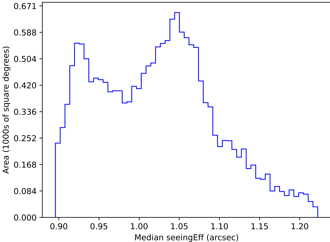
no_high_blob_v3.3_10yrs WFD all bands: Median seeingEff
