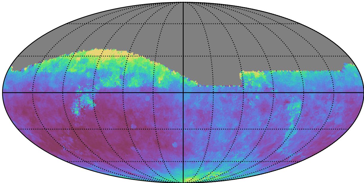
no_high_blob_v3.3_10yrs All sky z band: Median seeingEff
