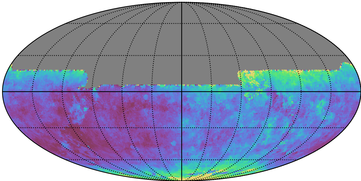
no_high_blob_v3.3_10yrs All sky y band: Median seeingEff
