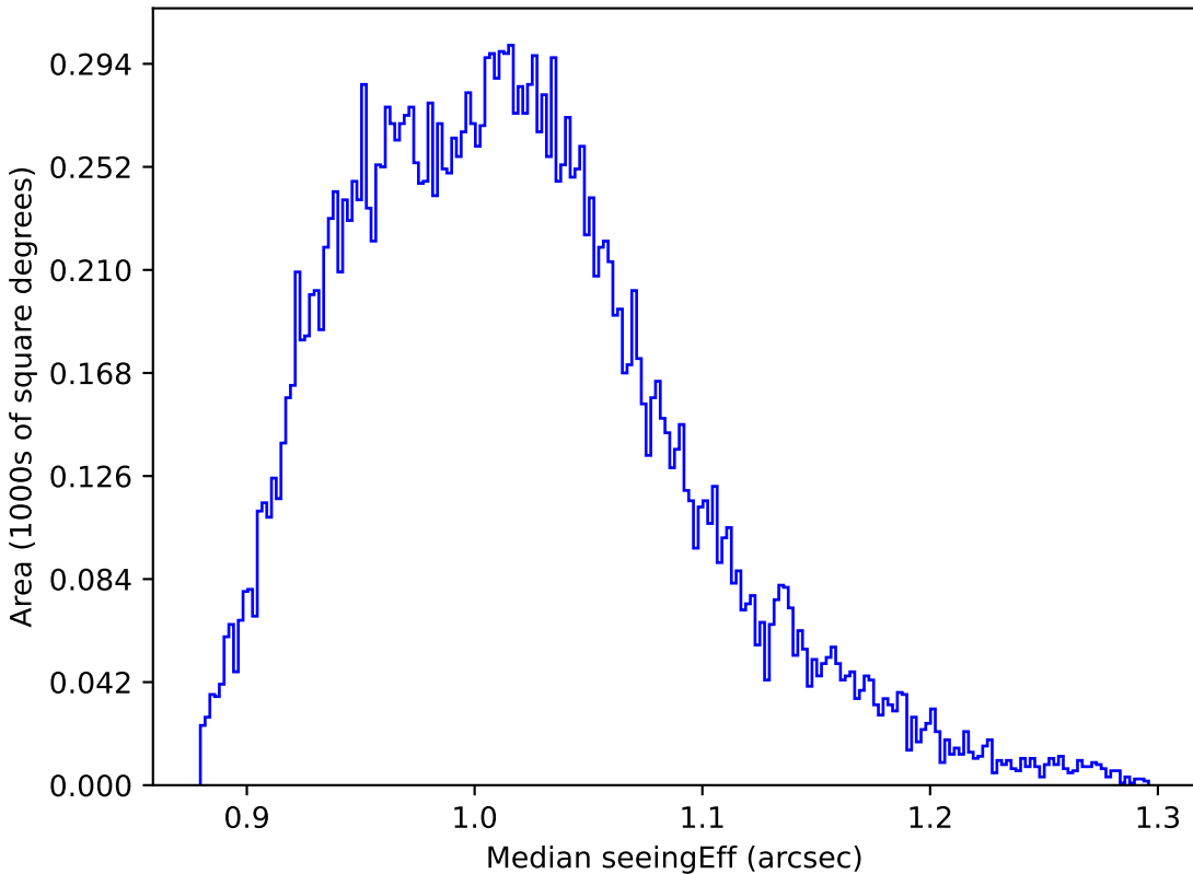
no_high_blob_v3.3_10yrs All sky y band: Median seeingEff
