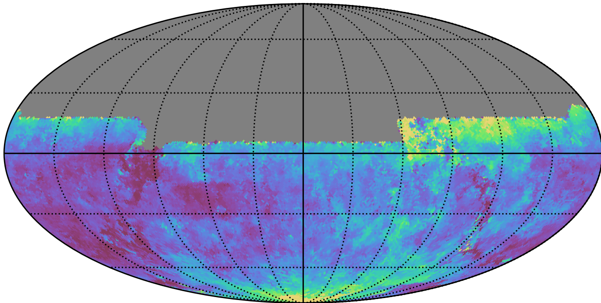
no_high_blob_v3.3_10yrs All sky u band: Median seeingEff
