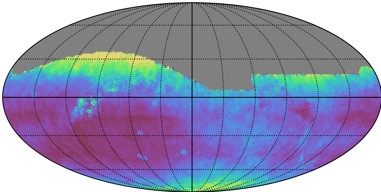
no_high_blob_v3.3_10yrs All sky r band: Median seeingEff
