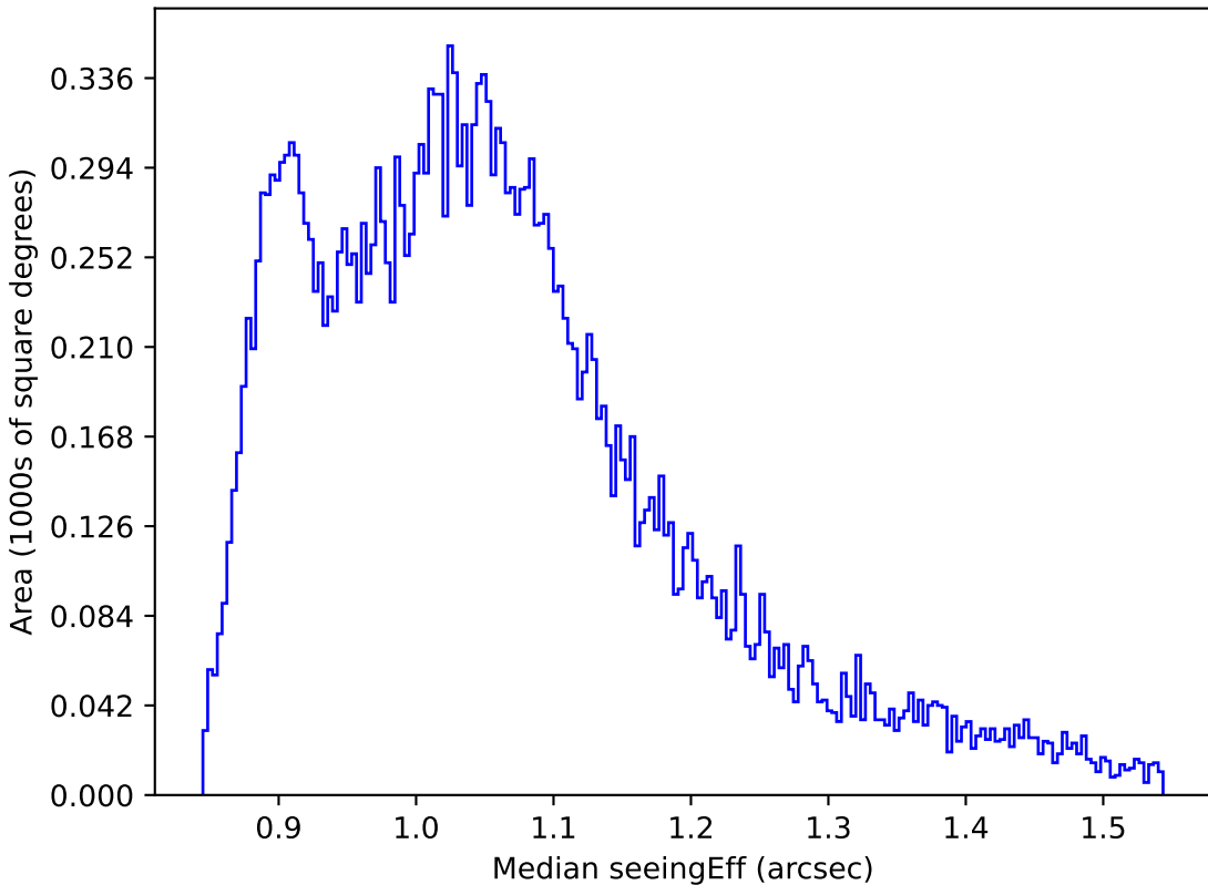
no_high_blob_v3.3_10yrs All sky r band: Median seeingEff
