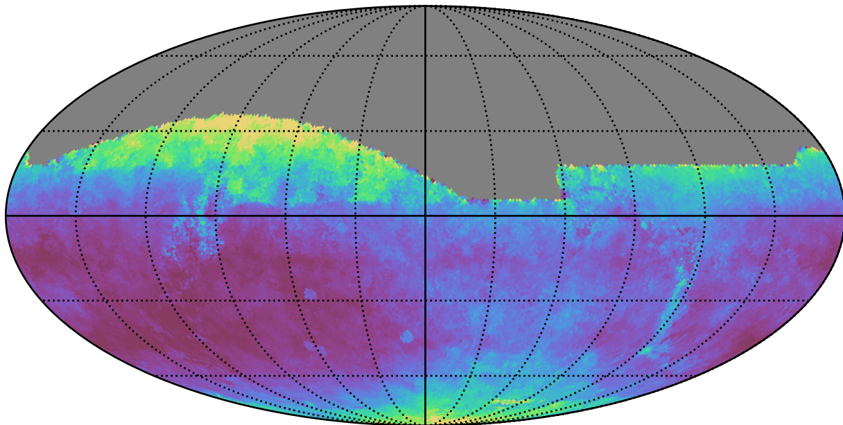
no_high_blob_v3.3_10yrs All sky i band: Median seeingEff
