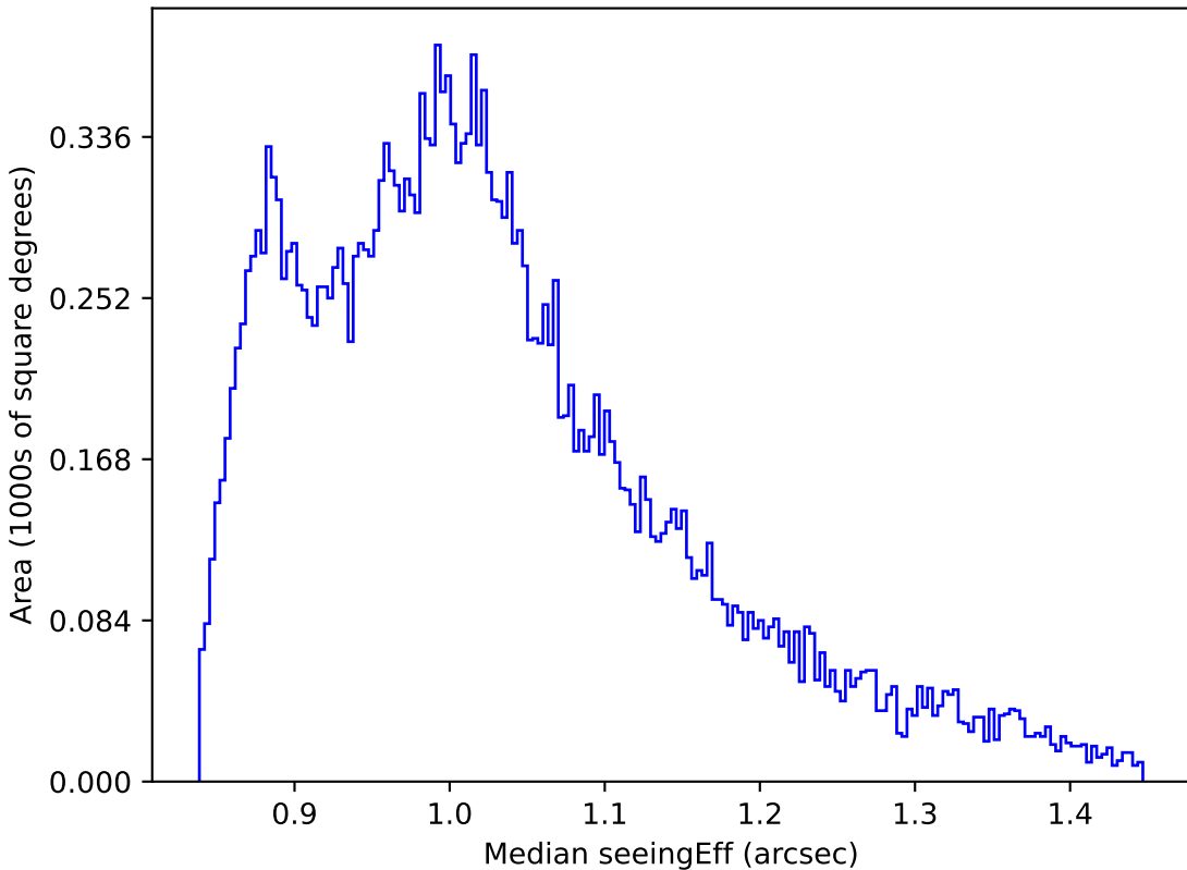
no_high_blob_v3.3_10yrs All sky i band: Median seeingEff
